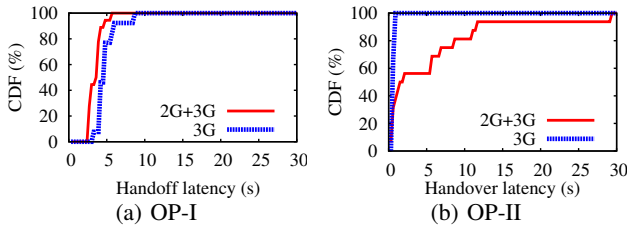
Figure 9: Active-state handoff latency in OP-I and OP-II in the 2G-blocking-3G case (C2) .
