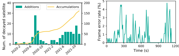
(a) Satellite failures (Starlink [35]) (b) Radio link failures (Tiantong) Figure 13: Intermittent failures in mobile satellites.
