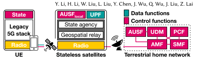
Figure 14: An overview of SpaceCore.
