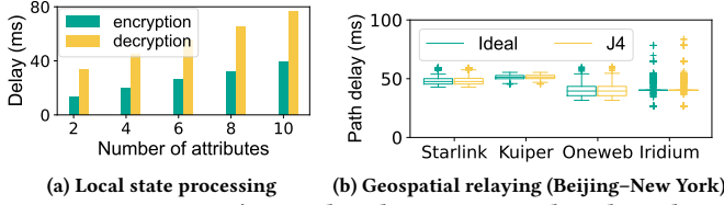
Figure 18: SpaceCore’s signaling latency micro-benchmark.
