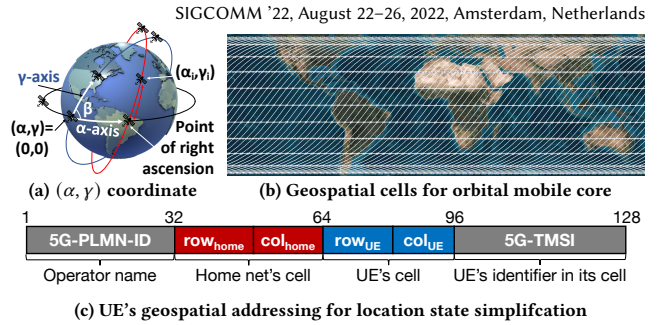
Figure 15: SpaceCore’s geospatial service area & state.
