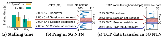
Figure 21: User-level performance in satellite mobility.
